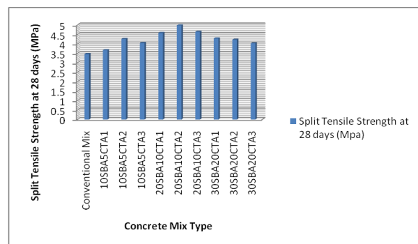
Fig 3.3: Graphical representation of split tensile strength at 28 days (MPa)
