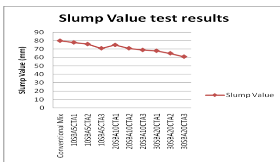
Fig 3.1: Graphical representation of slump value for different concrete mix
