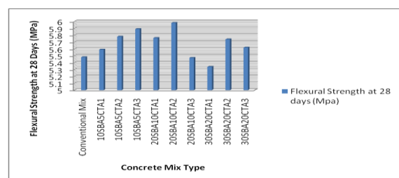
Fig 3.4: Graphical representation of Flexural strength at 28 days (MPa)
