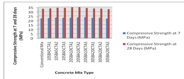
Fig 3.2: Graphical Representation of Compressive Strength at 7 and 28 days (Mpa)
